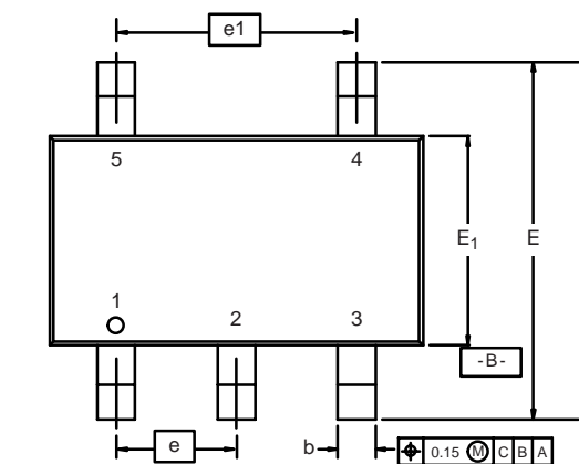
5-LEAD TSOP
