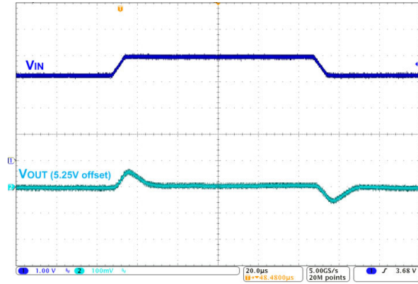
Figure 17. Line Transient, 3.2 <--> 3.9 V_{IN} , 7 µs Edge, 120 mA Load
