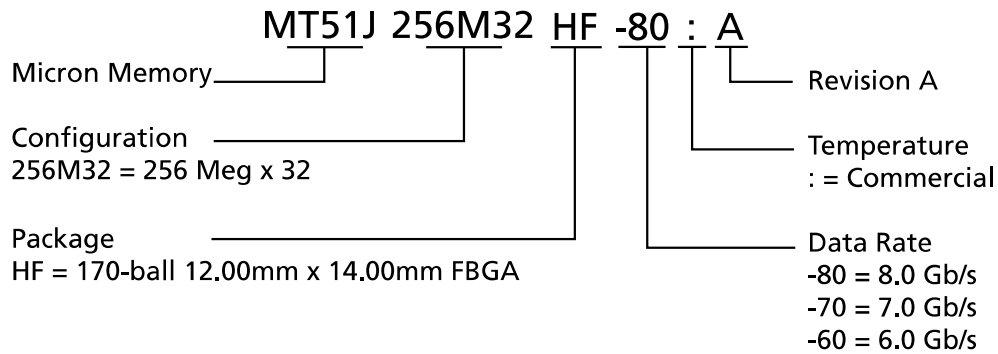
Figure 1: Part Numbering
