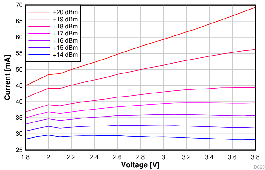
Figure 8-19. TX Current vs. Supply Voltage (VDD5) (50 kbps, 915 MHz)
