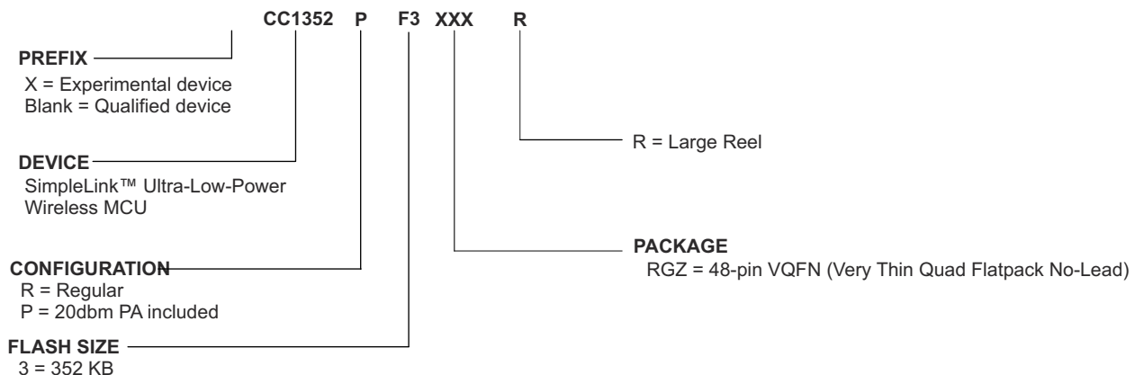
Figure 11-1. Device Nomenclature
