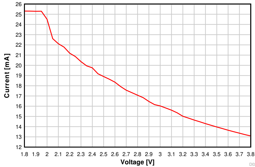
Figure 8-18. TX Current vs. Supply Voltage (VDD5) (50 kbps, 868.3 MHz)
