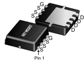
DFN3X3-8L (WDFN-8(3.3x3.3))
