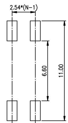
RECOMMENDED P.C.B. LAYOUT (TOP VIEW)
