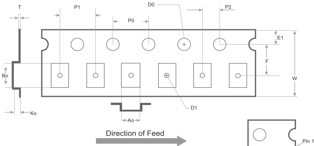
Figure 21 ▪ Tape and Reel Specifications for PE42546
