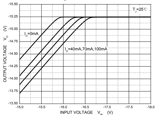
Dropout Characteristics
