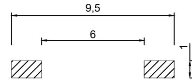
PCB. 焊接图 PCB. WELDING DRAWING
