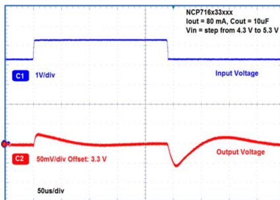
Figure 36. Line Transient Response
