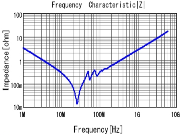
■ GRM31M5C2A473JA01 |Z| DC0V, 25degC
