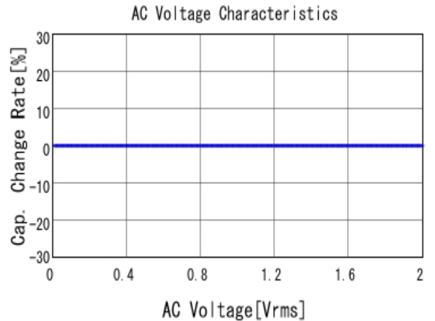
■ GRM31M5C2A473JA01 C-AC Voltage capchange, DC0V, 25.0d
