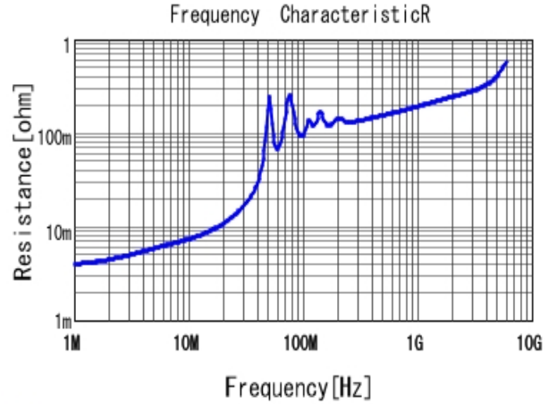
■ GRM31M5C2A473JA01 R DC0V, 25degC
