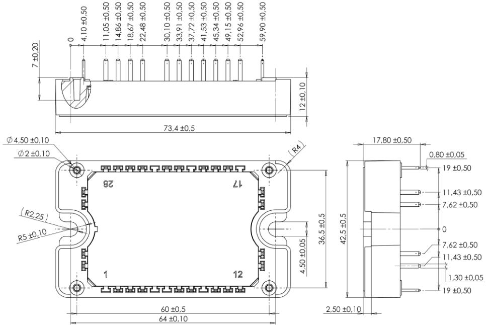
Figure 20 • Package Outline
