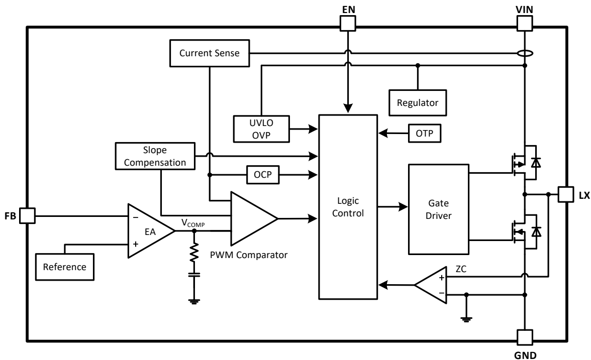
Figure 2. PAM2804 Block Diagram
