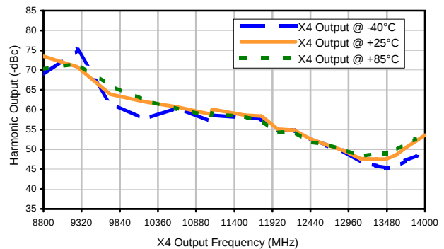
Harmonic X4 Output @ RF IN =7dBm
