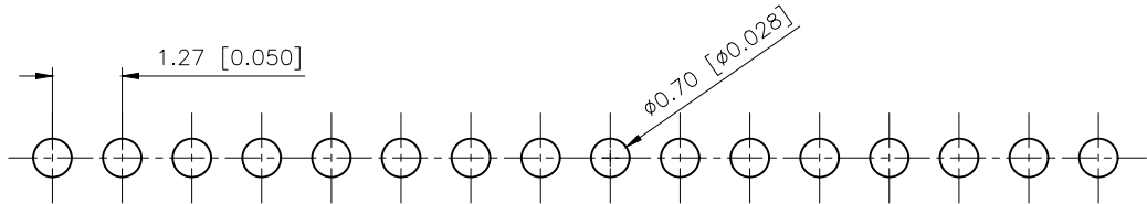
PCB LAYOUT
