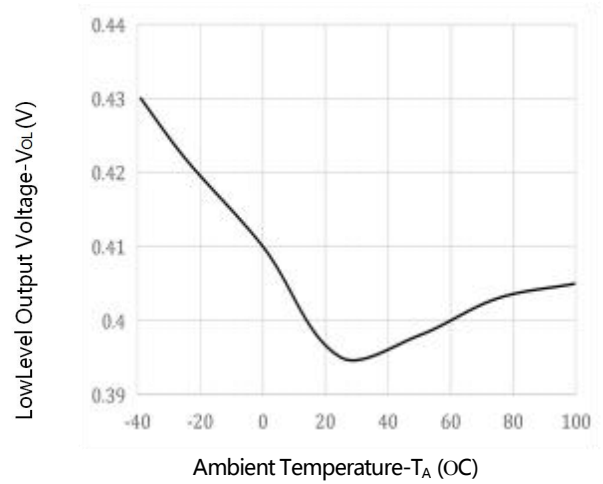
Fig.4 Low Level Output Voltage vs Ambient Temperature
