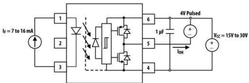
Figure17 I_{OH} Pulsed Test Circuit
