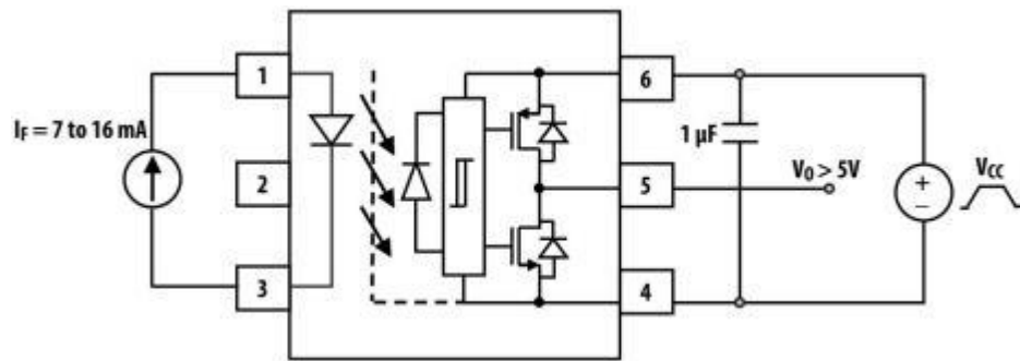
Figure 22 UVLO Test Circuit
