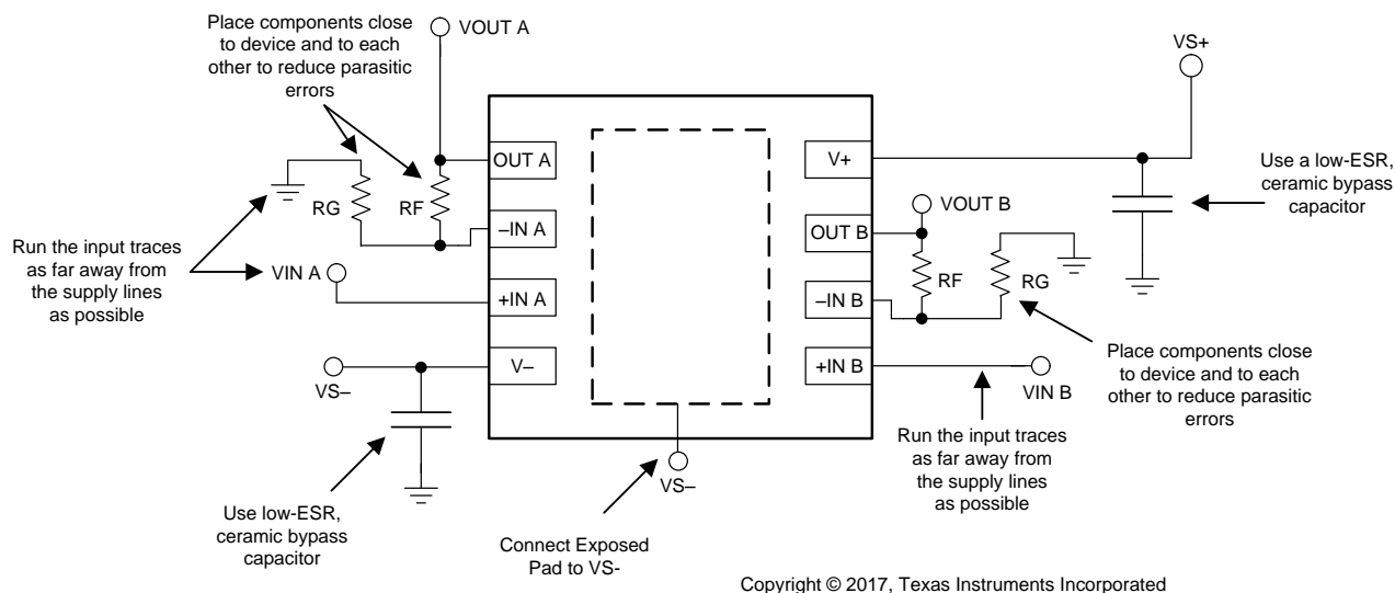
Figure 29. Layout Example
