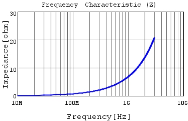
LQP03TN1N1B02 |Z|
