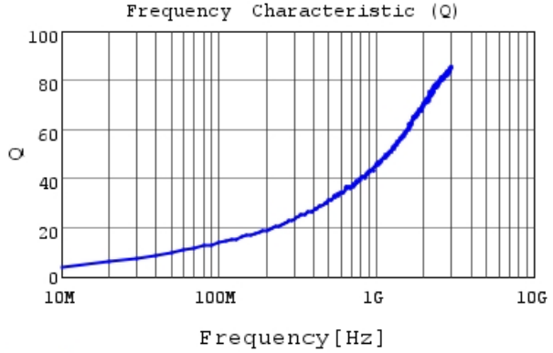
LQP03TN1N1B02 Q
