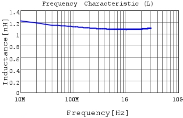
LQP03TN1N1B02 L
