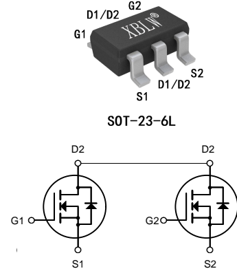
Dual N-Channel MOSFET
