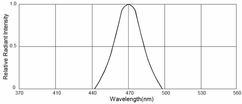
Fig.1 Relative Radiant Intensity VS. Wavelength
