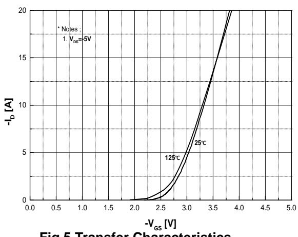
Fig.5 Transfer Characteristics
