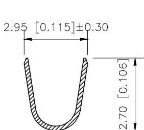
SECTION:A-A SCALE:1:1
