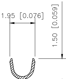
SECTION:B-B SCALE:1:1
