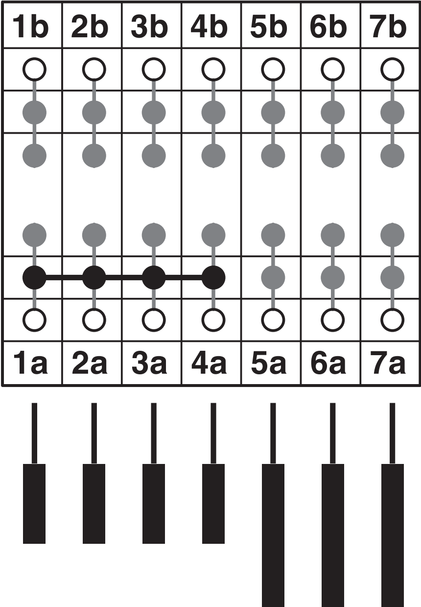
Circuit diagram
