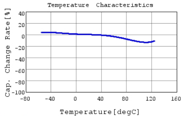
GRM32DR72J473KW01 C-Temp. capchange, DCOV, 1
