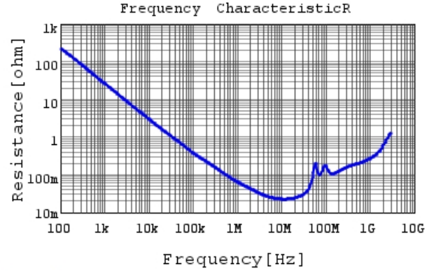
GRM32DR72J473KW01 R DCOV, 25degC
