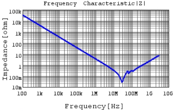
GRM32DR72J473KW01 |Z| DCOV, 25degC
