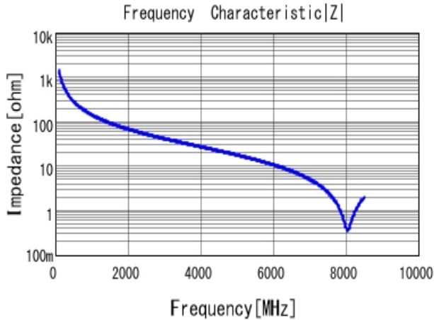
■ GJM1555C1H1R1BB01 |Z| DC0V, 25degC
