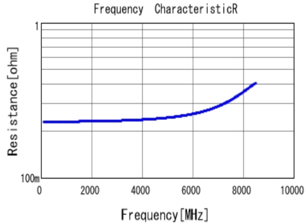
■ GJM1555C1H1R1BB01 R DC0V, 25degC
