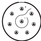
18-08 8 contacts size 12
