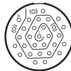
18-31 31 contacts size 20
