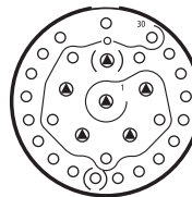
22-30 24 contacts size 20 6 contacts size 12
