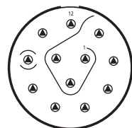
22-12 12 contacts size 12
