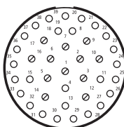
22-39 27 contacts size 20 12 contacts size 16
