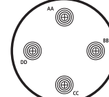
20-04 4 contacts K6
