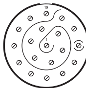
22-19 19 contacts size 16
