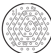
22-55 55 contacts size 20
