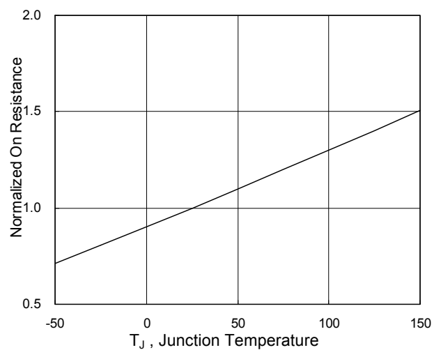
( ^\circ C ) Fig.6 Normalized R_{DSON}
