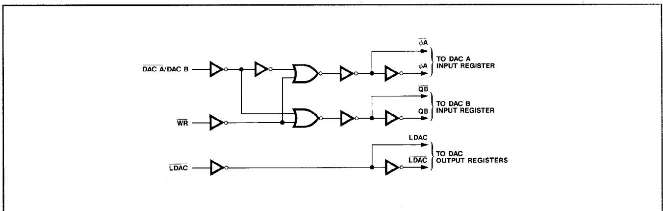
FIGURE 4: Input Control Logic
