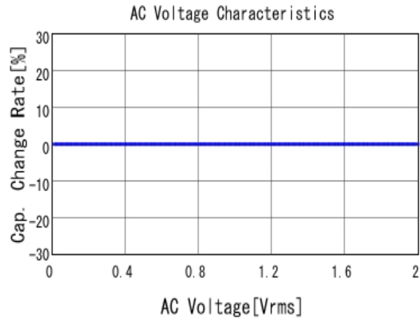
■ GRM0332C1H680GA01 C-AC Voltage capchange, DC0V, 20.0d
