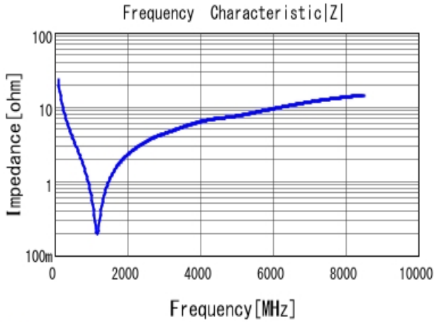
■ GRM0332C1H680GA01 |Z| DC0V, 20degC
