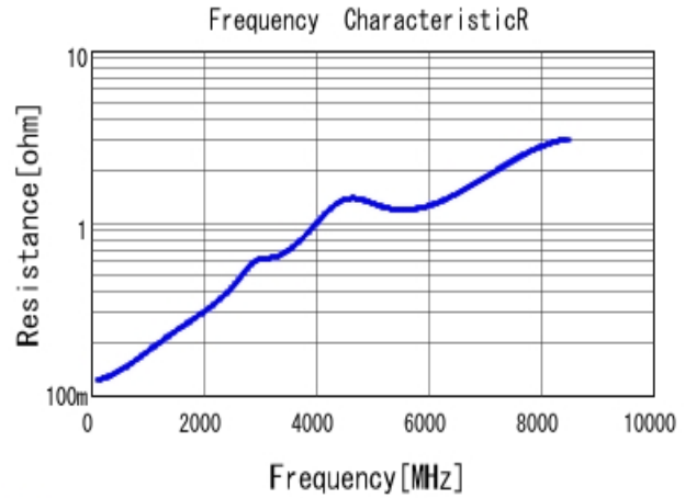
■ GRM0332C1H680GA01 R DC0V, 20degC
