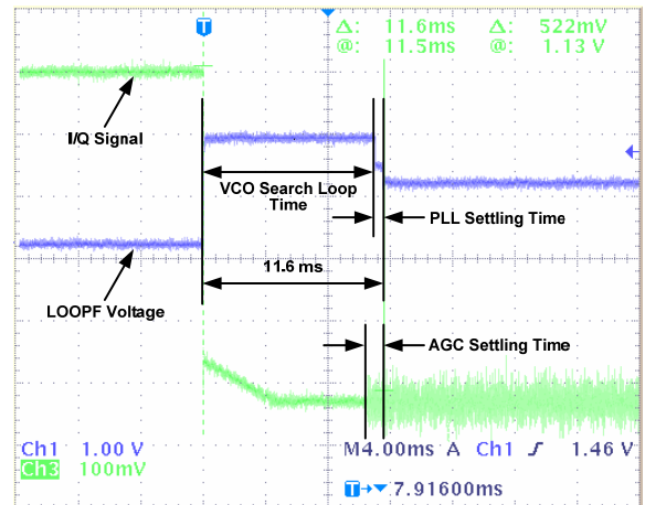
Figure 20. Software Power ON Timing
