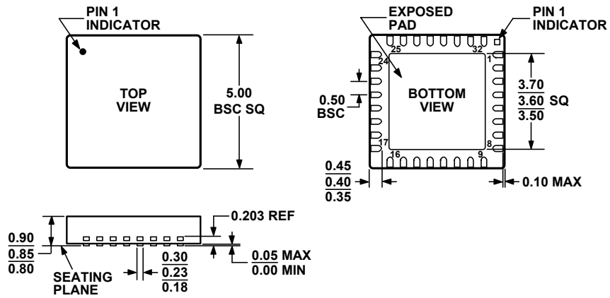
Figure 41. 32-Lead QFN Package 5 mm × 5 mm Body (CP-32) Dimensions shown in millimeters
