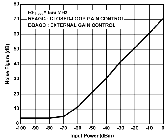
Figure 7. UHF Noise Figure vs. Input Power
