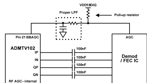
Figure 34. AGC Connection
