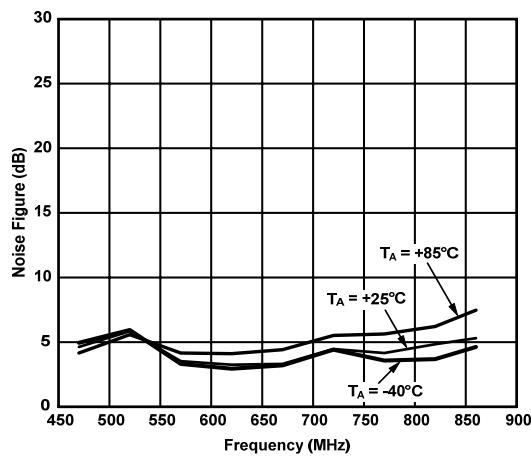
Figure 6. UHF Noise Figure vs. Frequency
