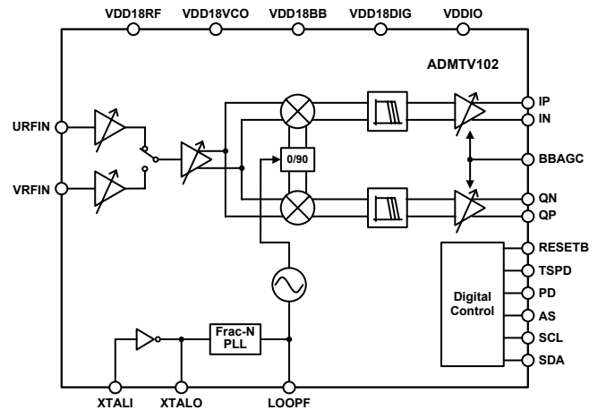
Figure 1. Block Diagram
