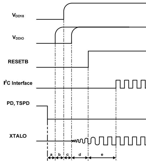
Figure 2. Digital Timing Diagram
