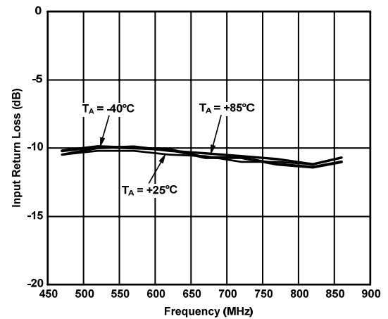
Figure 8. UHF Input Return Loss vs. Frequency [LNA Gain Mode: High]
