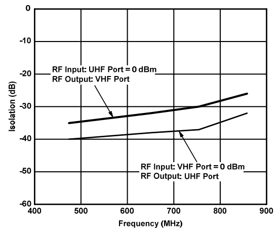
Figure 15. Port-to-Port Isolation
