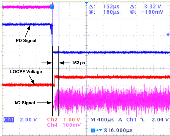
Figure 22. Hardware Power ON Timing
