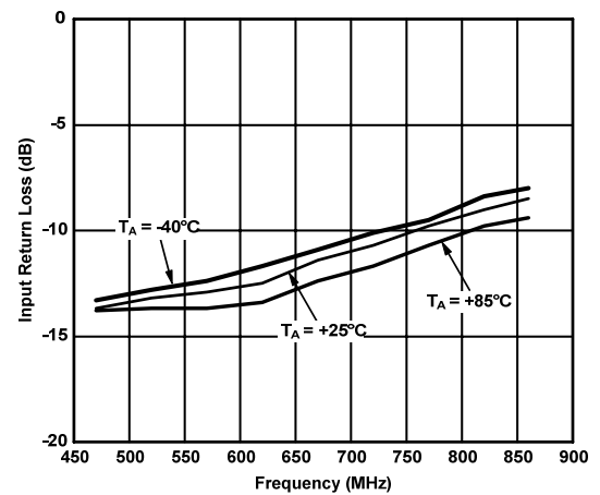
Figure 9. UHF Input Return Loss vs. Frequency [LNA Gain Mode: Low]
