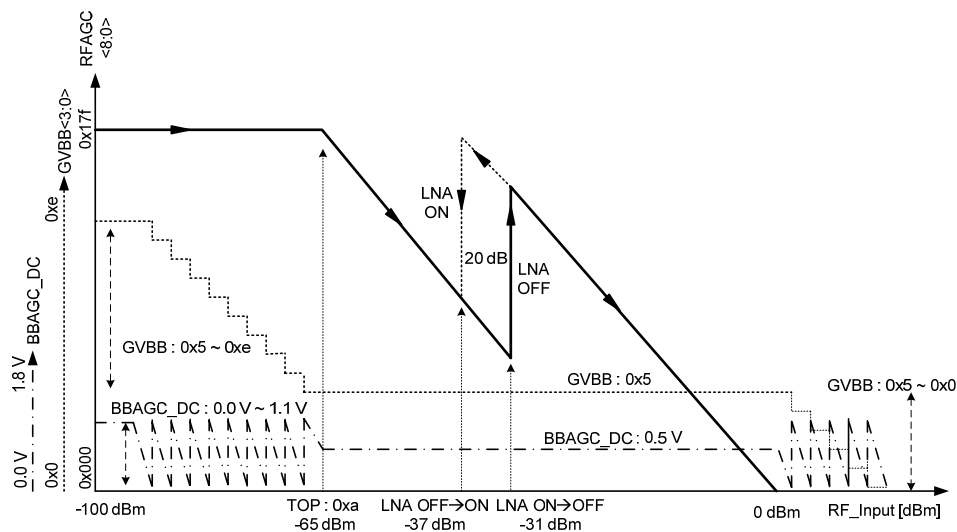
Figure 27. RFRSSI Graph
