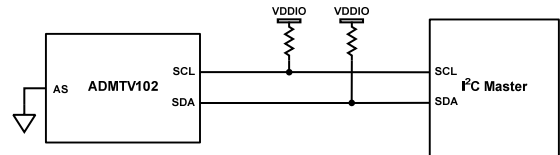
Figure 32. I 2 C Interface between ADMTV102 and I 2 C Controller
