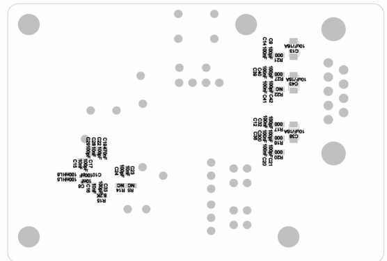
Figure 39. Evaluation Board Silkscreen Bottom View
