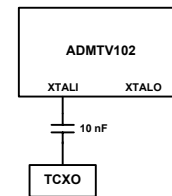
Figure 35. TCXO Application
