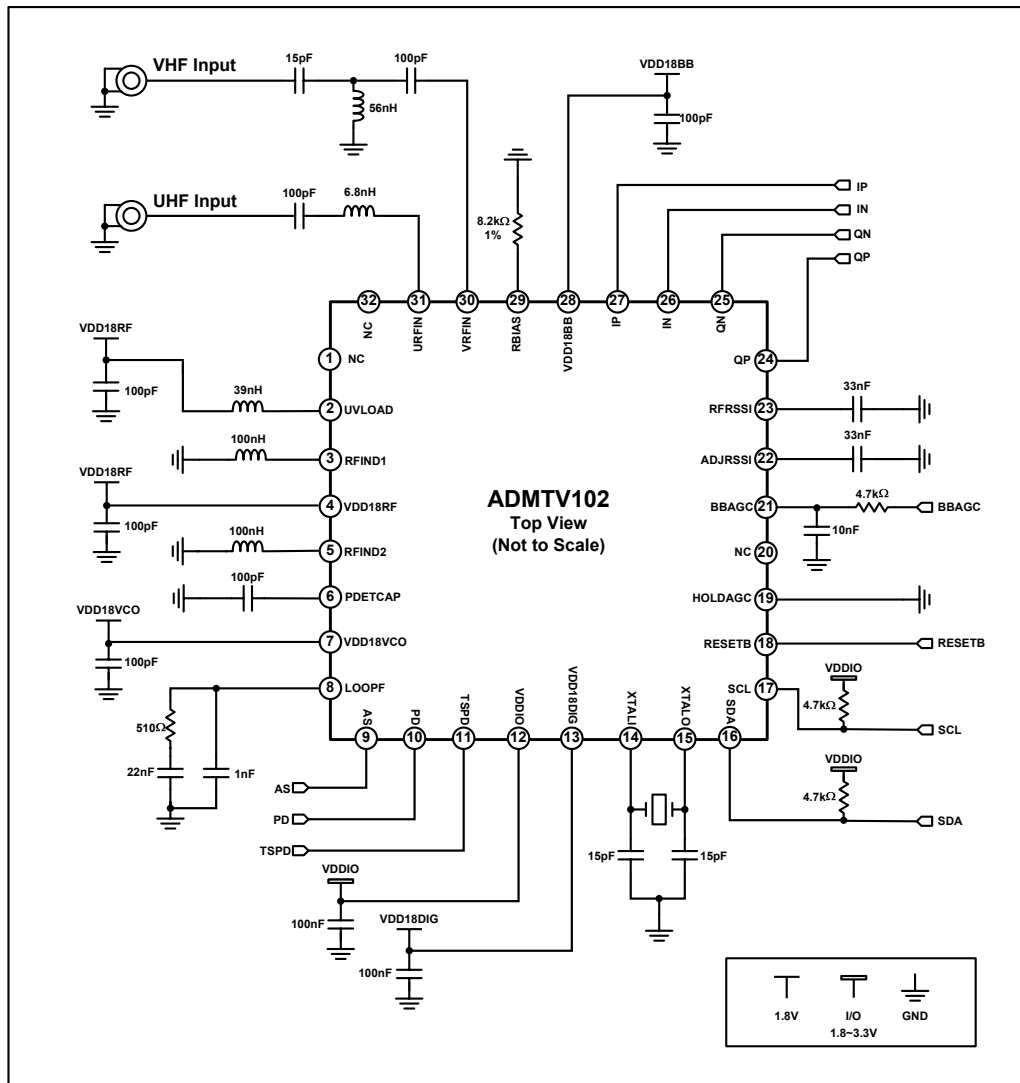
Figure 28. Application Schematic
