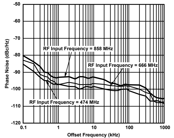
Figure 14. UHF Phase Noise vs. Offset Frequency
