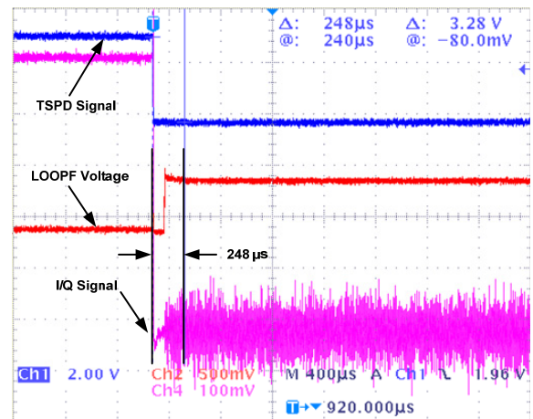
Figure 21. Time-slicing Power ON Timing
