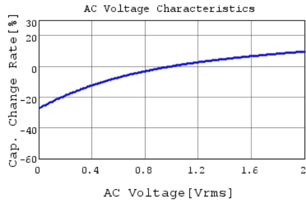
GRM21BZ71H475KE15 C-AC Voltage capchange, Dc
