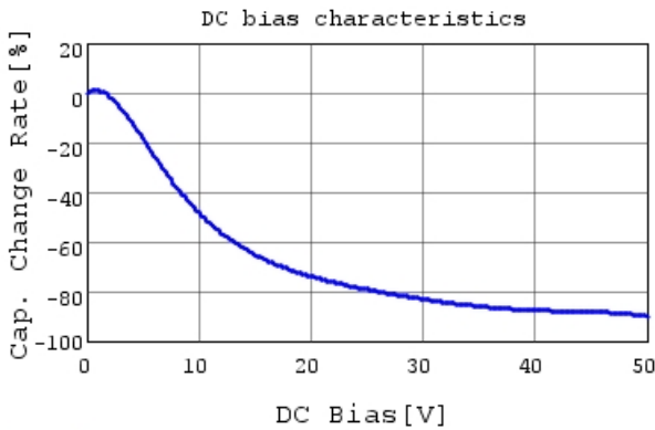
GRM21BZ71H475KE15 C-DC bias capchange, 25.0c
