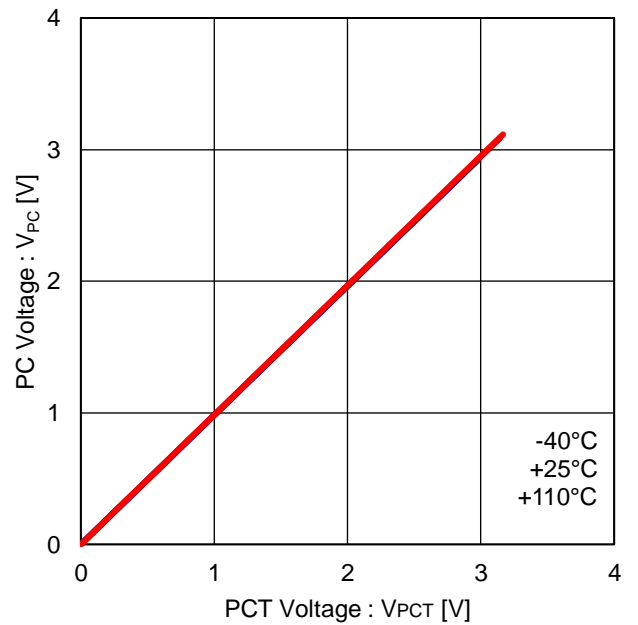
Figure 33. PCT vs PC Linearity ( R_{PCT}=R_{PC}=100k\Omega )
