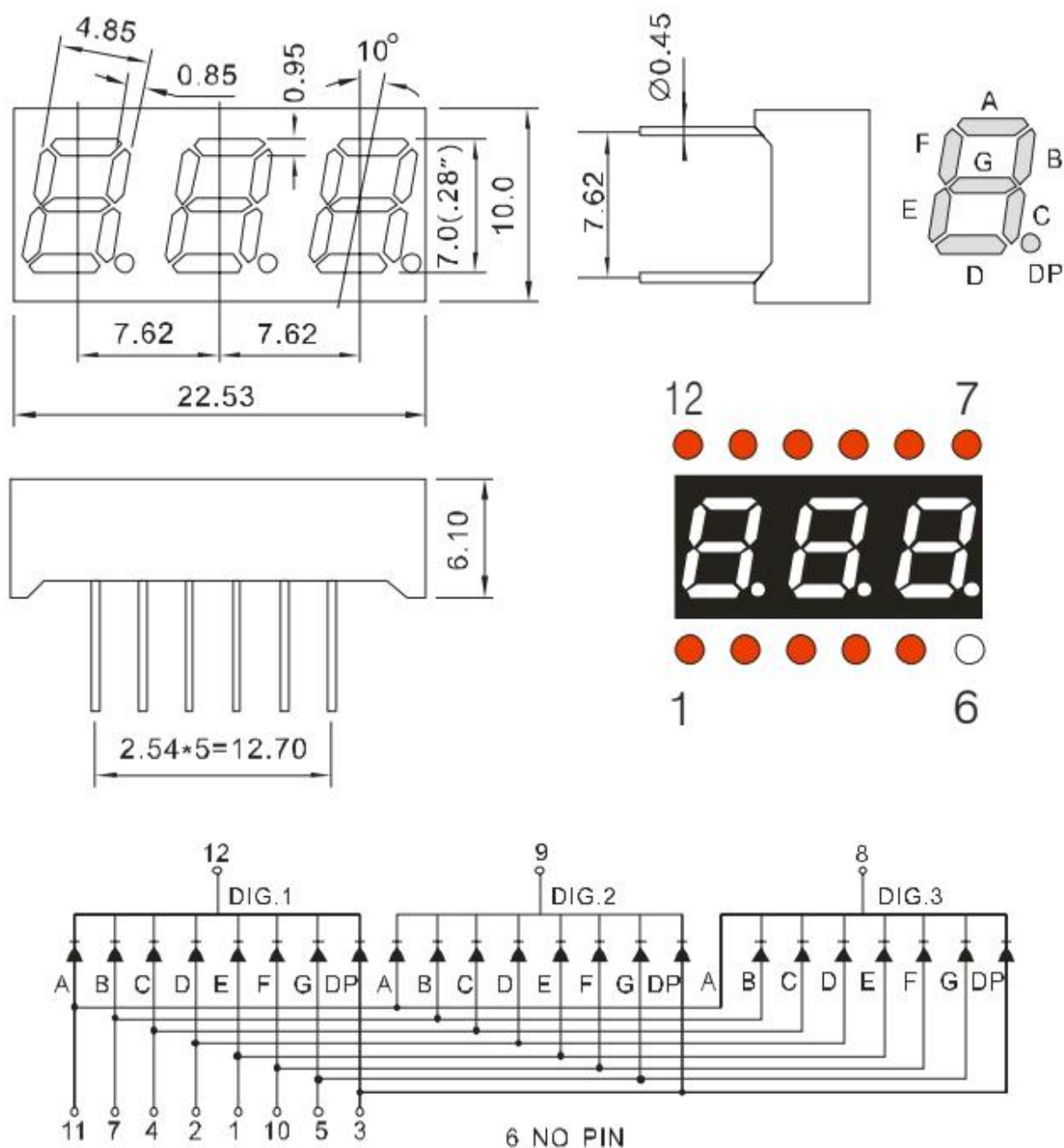
Figure Size & Circuit Principle Diagram : 22.53mm×10.0mm×6.1mm
