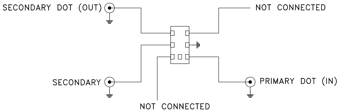
Schematic Diagram
