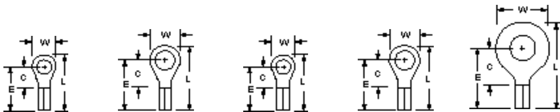
MU18-6RHT/S MU18-10RHT MU14-6RHT/S MU14-10RHT MU14-14RHT Stud Size 6 10 6 10 1/4 Wire Range 22-18 22-18 16-14 16-14 16-14
