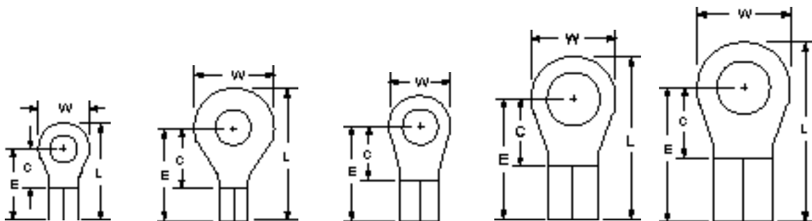
MU10-10RHT MU10-14RHT MU8-14RHT/S MU6-38RHT MU4-38RHT Stud Size 10 1/4 1/4 3/8 3/8 Wire Range 12-10 12-10 8 6 4
