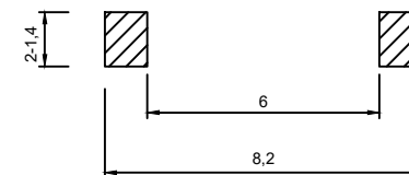
PCB. 焊接图 PCB. WELDING DRAWING
