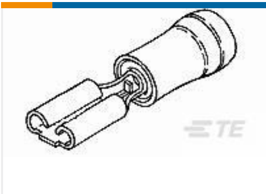
TE Part #61060-1 RECEPT,PIDG FASTON 22-18 110
