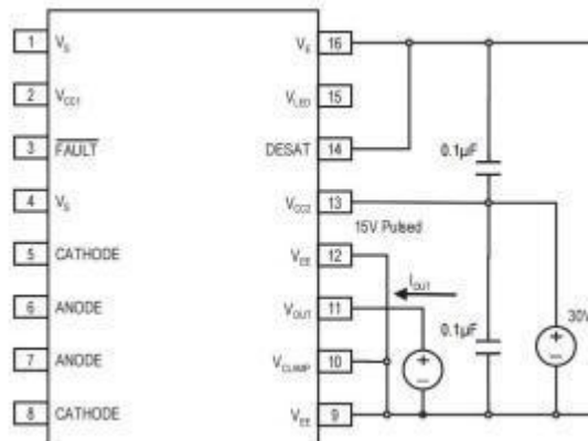
Figure 24. V_{OL} Pulsed Test circuit
