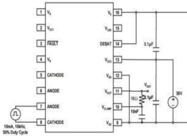
Figure 29. T_{PLH} , T_{PHL} , T_i , T_r Test circuit
