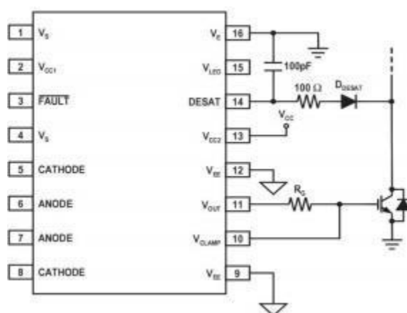
Figure 38. DESAT pin protection
