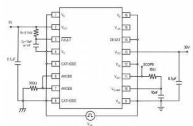
Figure 33. CMR Test Circuit LED1 on
