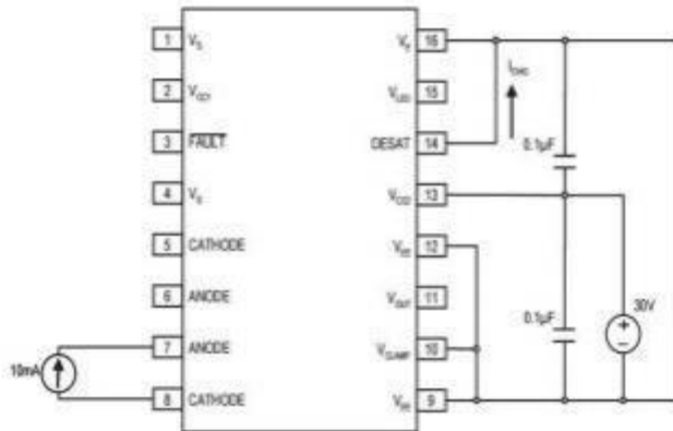
Figure 27. I_{LHG} Pulsed Test circuit
