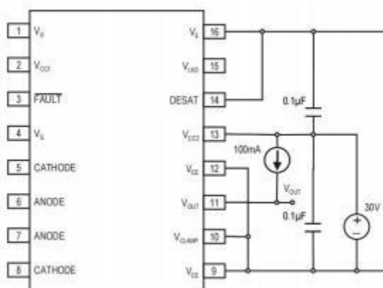
Figure 26. I_{cc2L} Test circuit
