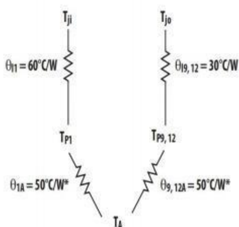
Figure. 41 AT333J thermal model
