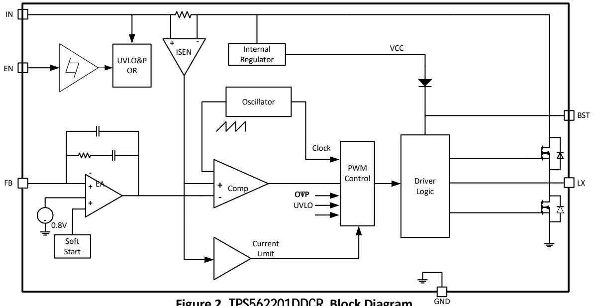
Figure 2. TPS562201DDCR Block Diagram
