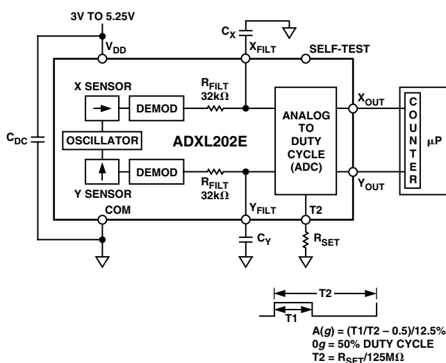
Figure 3. Block Diagram
