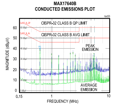
CONDITIONS: V_{IN} = 24V , V_{OUT} = 5V , I_{OUT} = 0.4A MEASURED ON THE MAX17640BEVKIT# WITH L201 = 22\mu H , C202 = C204 = 1\mu F/100V/X7R/1206
