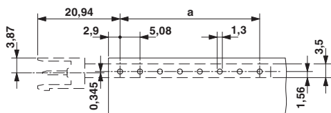
Drilling diagram
