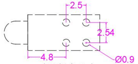
建议焊盘尺寸 Recommended Soldering Pattern
