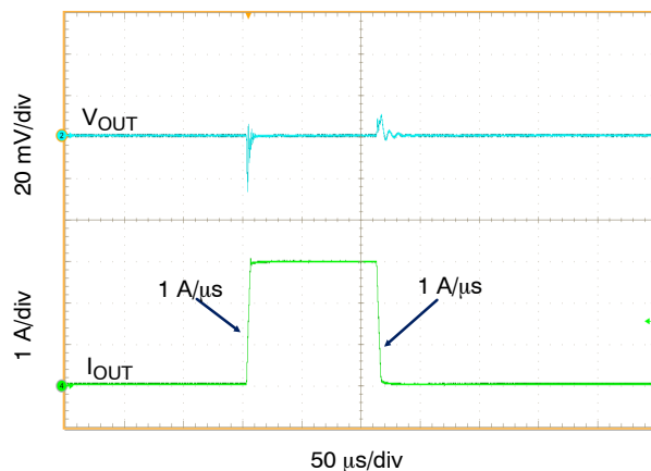
Figure 8. Load Transient Response, I_{OUT} = 10\text{ mA} to 3\text{ A} , C_{OUT} = 10\text{ }\mu\text{F MLCC}
