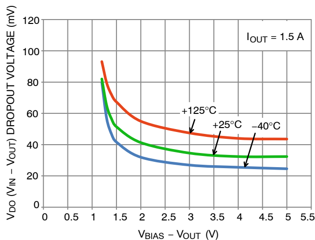
Figure 4. V_{IN} Dropout Voltage vs. (V_{BIAS} - V_{OUT}) and Temperature T_J
