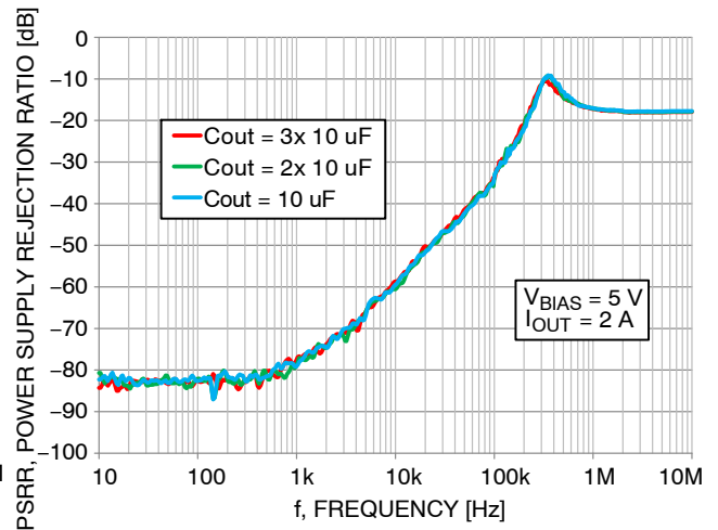
Figure 22. V_{BIAS} Power Supply Rejection Ratio vs. Frequency
