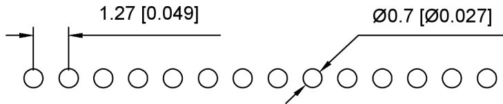
PCB LAYOUT
