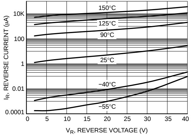
Figure 6. Leakage Current
