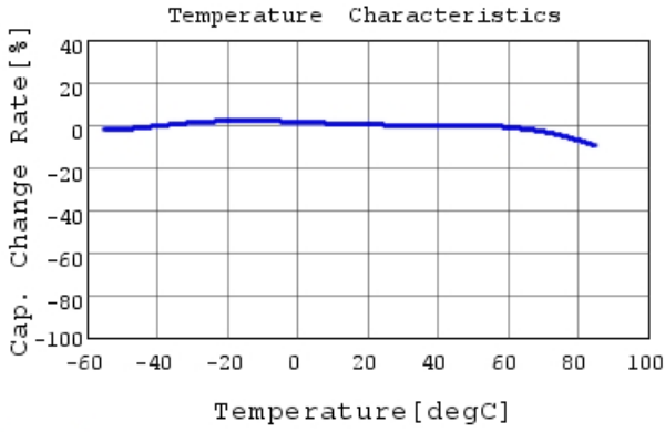
GRM155R61A105KE01 C-Temp. capchange, DC0.0V,
