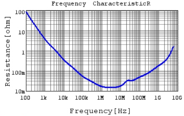
GRM155R61A105KE01 R DCOV, 25degC
