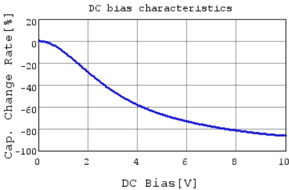
GRM155R61A105KE01 C-DC bias capchange, 25.0c
