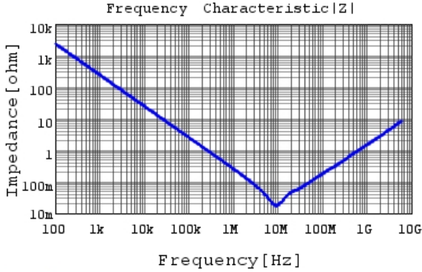
GRM155R61A105KE01 |Z| DCOV, 25degC
