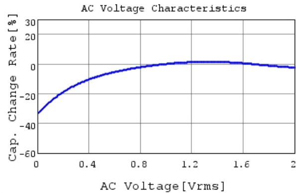
GRM155R61A105KE01 C-AC Voltage capchange, Dc
