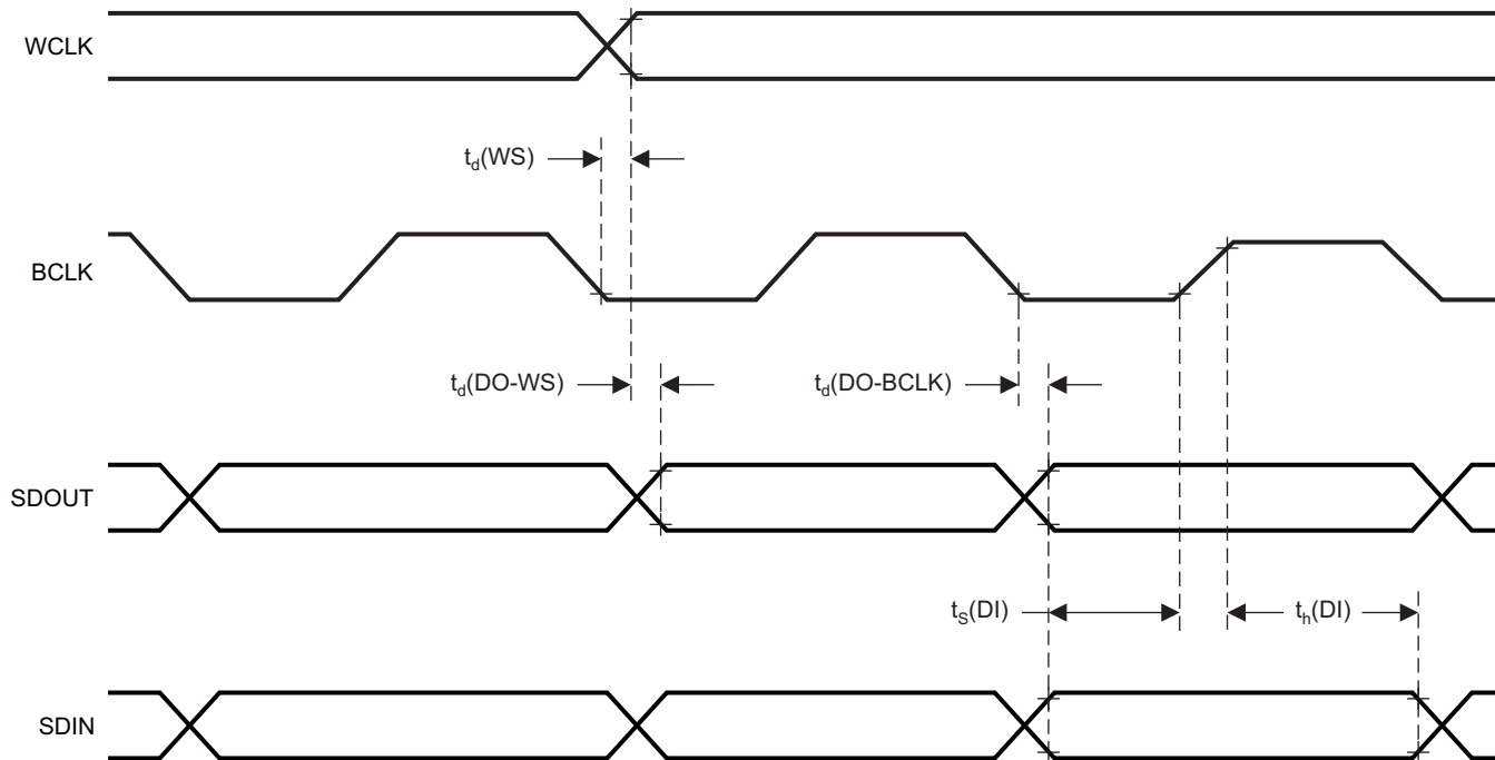
Figure 1. I 2 S, Left-Justified and Right-Justified Format Timing in Master Mode
