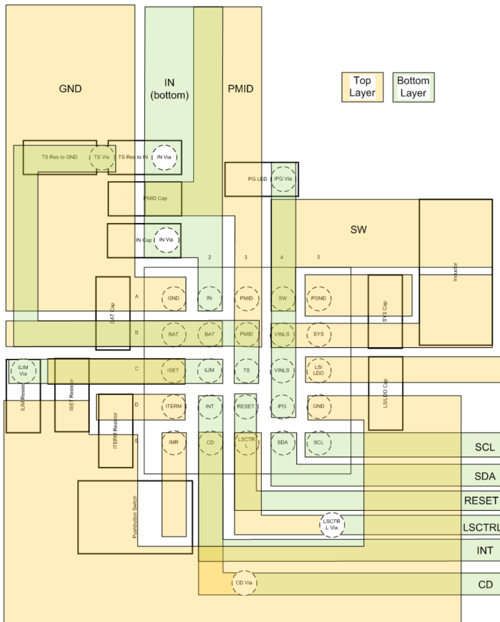
Figure 105. bq25122 Layout
