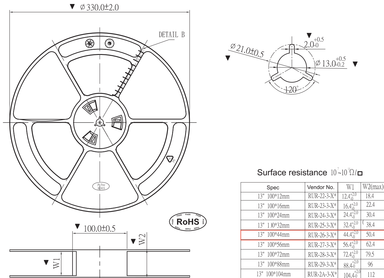
Figure 10-1. Tape Specification
