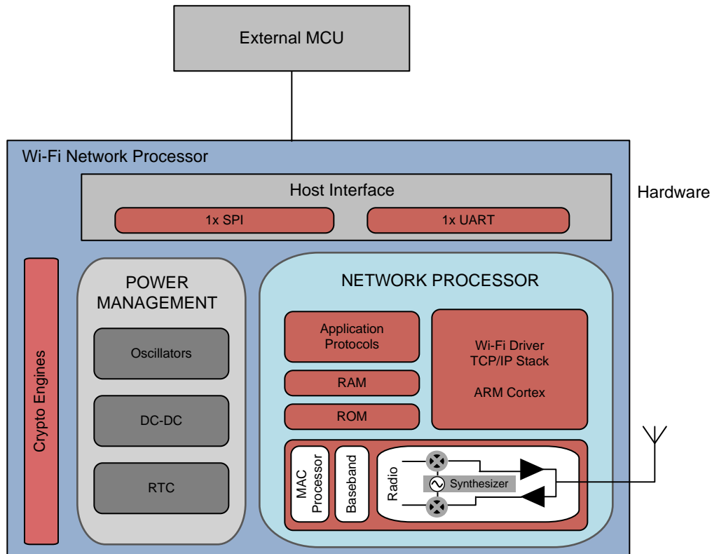
Figure 1-2. CC3120 Hardware Overview
