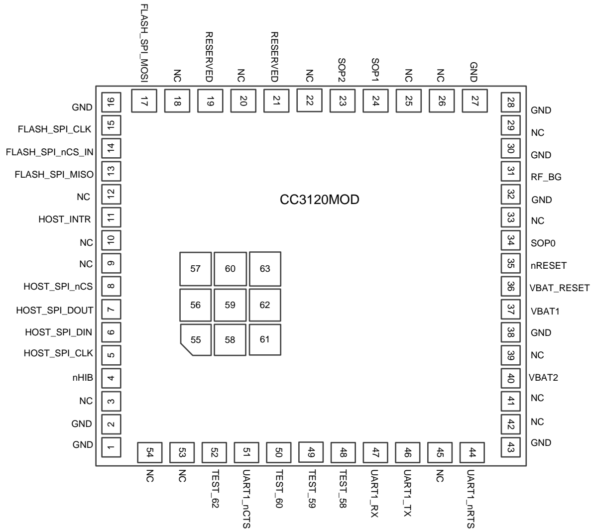
Figure 4-1. CC3120MOD Pin Diagram Bottom View
