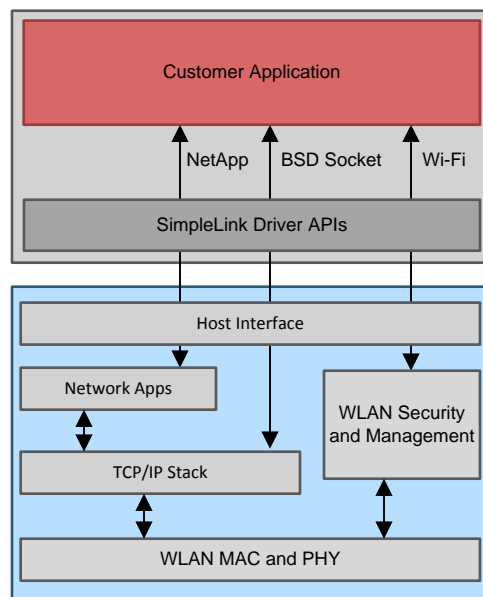
Figure 1-3. CC3120 Embedded Software Overview
